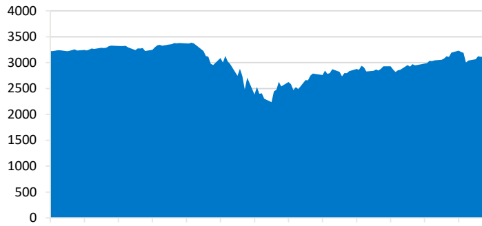
S&amp;P 500 Index: Trailing 180 Days
